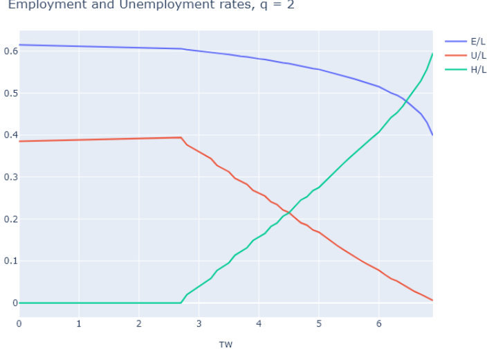
Figure 19: Employment, Unemployment and Self production rates for changes in Transport Costs with DRS
