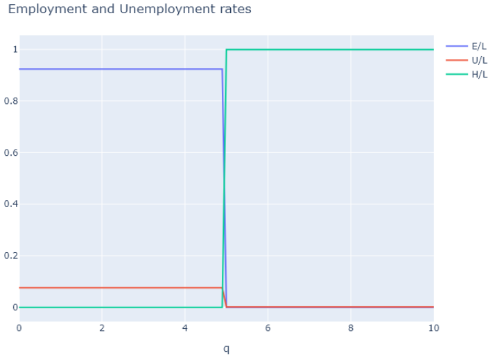
Figure 17: Impact of q on Employment Rates
