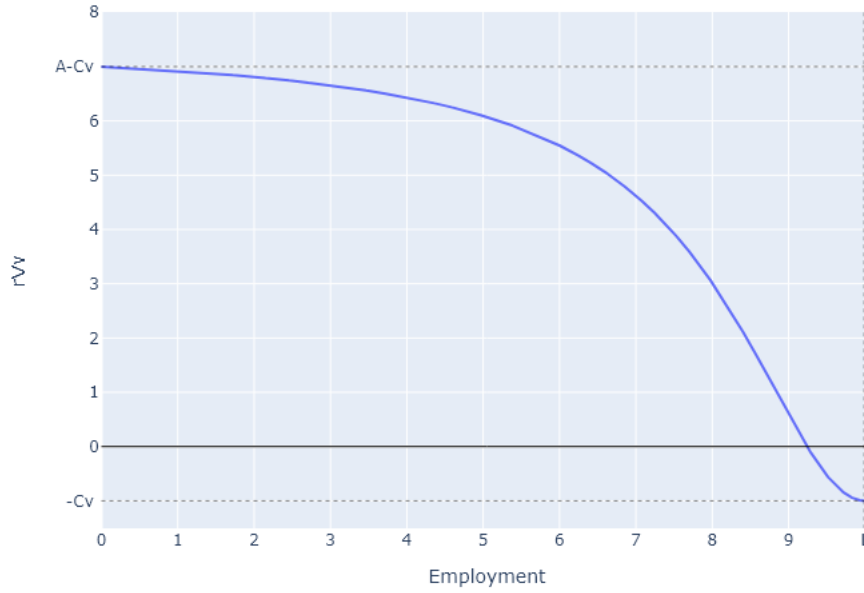
Figure 6: Equilibrium employment in the search model
