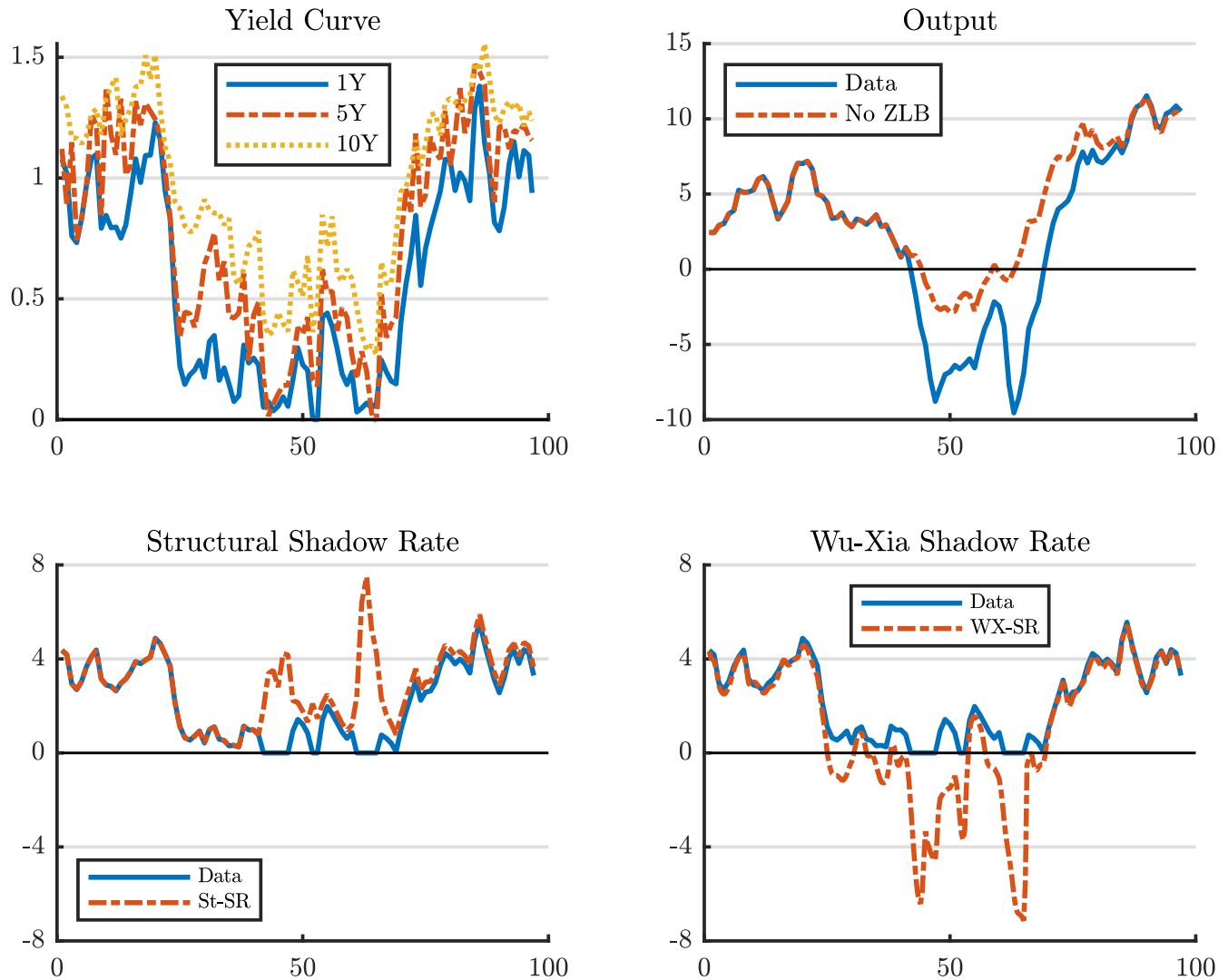
Figure D.2: Simulation to Compare Different Approaches to Measuring the Shadow Rate
