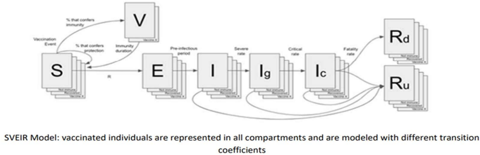
Figure 1. SVEIR model
